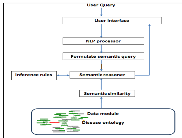
Fig.4. Proposed architecture for SDA.
