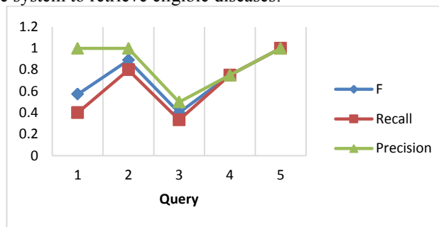
Fig. 2. Shows the precision, recall and F-measures of SDA on 5 queries from the query set
